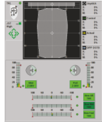
Port Engine Lost
